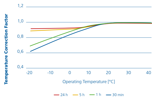
Temperature Correction Factor vs Discharge rates
