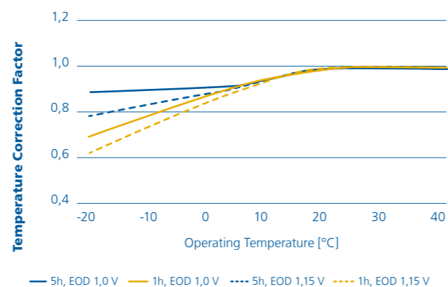
Temperature Correction Factor vs EOD Voltage
