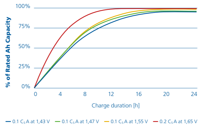
Rechargeability of GAZ® Lomain KGL cells at +20 °C
