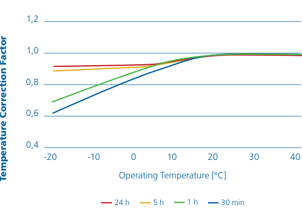
Temperature Correction Factor vs Discharge rates
