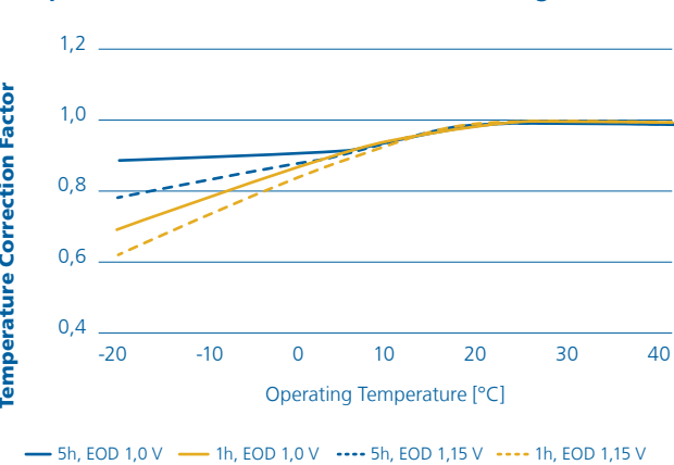
Temperature Correction Factor vs EOD Voltage
